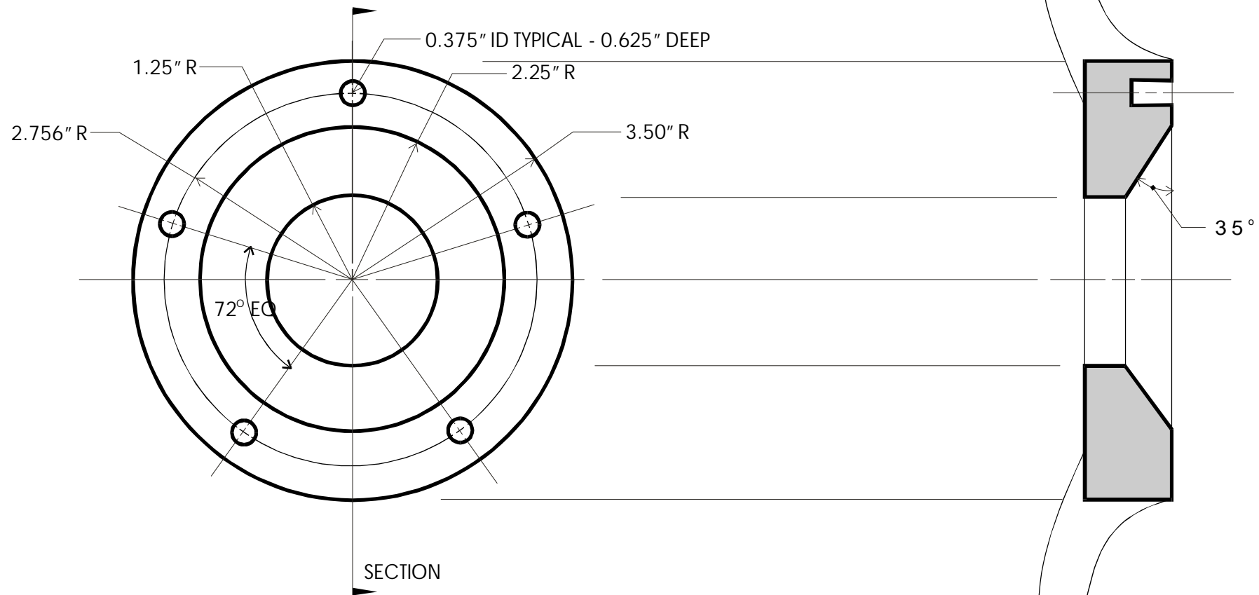
SECTION
